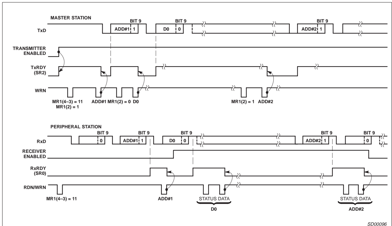
Figure 12. Wake-Up Mode
